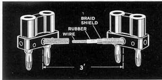
Type 274-NC Shielded Conductor
