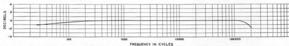
Frequency characteristic TYPE 741-P Plate-to-Line Transformer. Voltage step-down ratio 6.35:1
