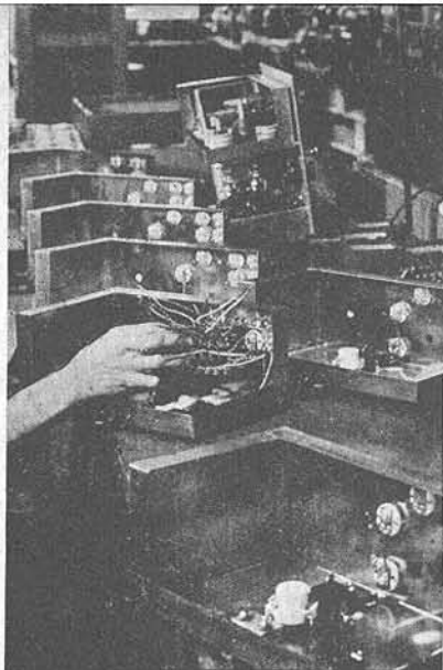
20 - ASSEMBLING OSCILLATOR SHELVES.
