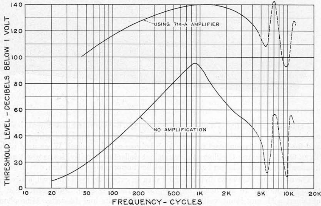
Frequency characteristic of a TYPE 714-A Amplifier
