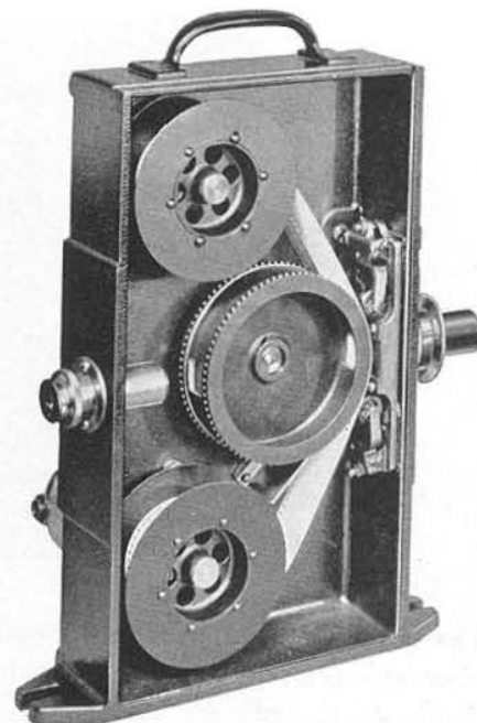
Interior View of the High-Speed Camera
