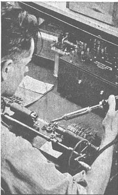
5 - WINDING ATTENUATOR RESISTANCES
