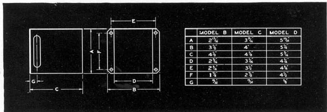
Dimensions for standard General Radio transformer-mounting cases
