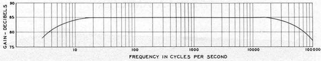
Frequency characteristic of a TYPE 714-A Amplifier
