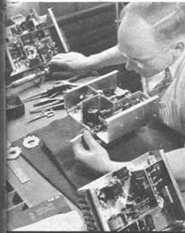
13 - WIRING AMPLIFIER SHELF ASSEMBLY
